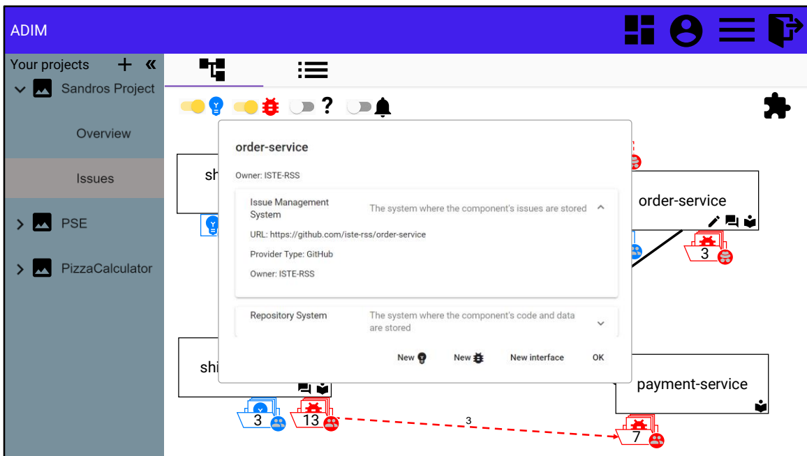
Dialog with information of a component.
