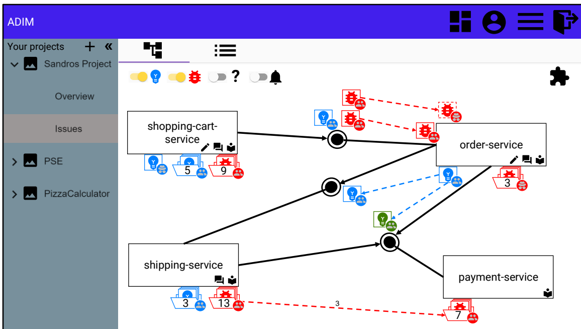
Component view showing all open feature requests and bugs
