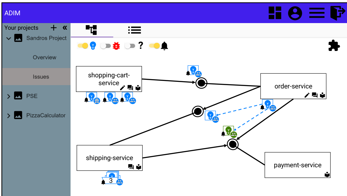
Component view showing only feature requests with a notification for the system user
