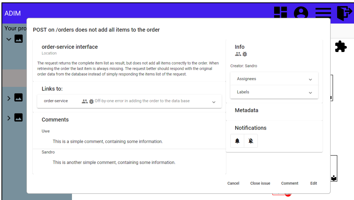
Issue Dialog with information about the issue. In this case a public Bug-Report
